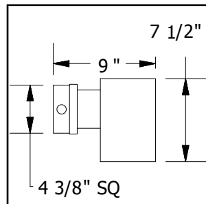
-38 J-Box Option
